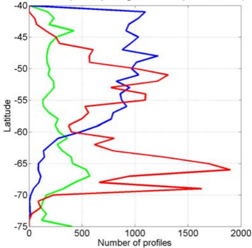
Number of profiles per degree Latitude (south of 40° S)
