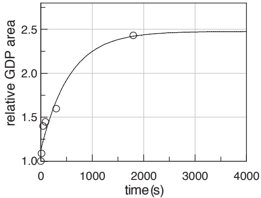
HPLC assay
