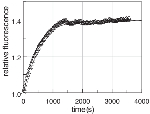
Fluorescence assay
