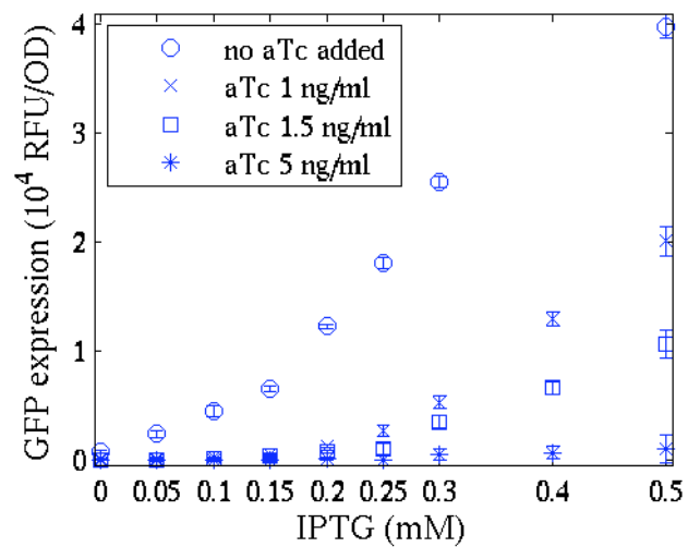
Figure S3. Example for raw data, used to compile Fig. 2a of the main text. “GFP expression” for strains (ZZS23) harboring P_{L_{tet-01}}:ryhB on a plasmid, in addition to the P_{L_{lac-01}}:crsodB-gfp reporter. The IPTG dependence of GFP expression (defined from plots such as Figure S2) is plotted for different degrees of RyhB expression. The latter is controlled by the level of the inducer aTc in the growth medium as indicated by the legend.
