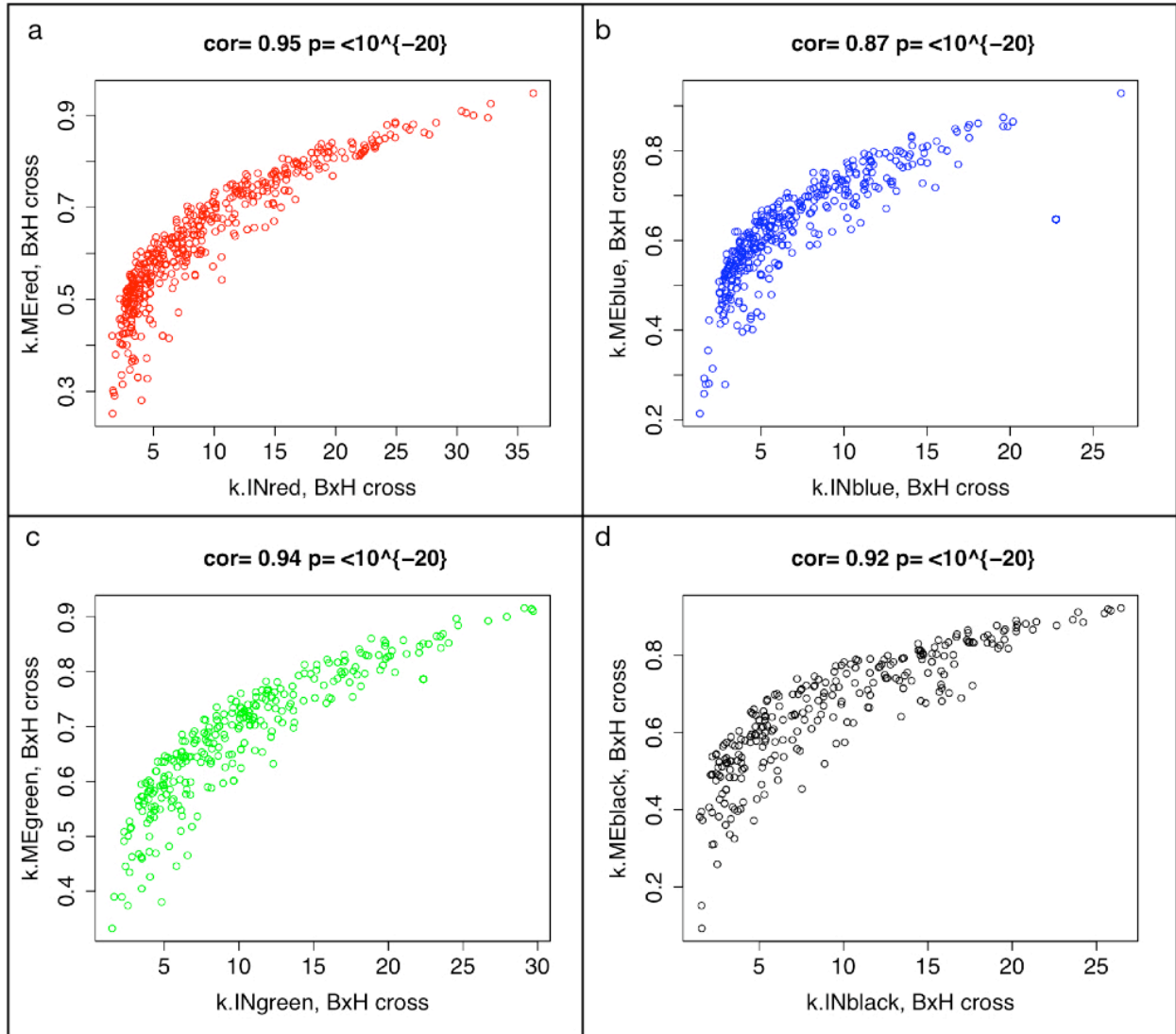
Supplementary Fig. 1: Scatterplots of kIN (intramodular connectivity) and kME (module eigengene-based connectivity) in the four largest modules of the BxH data: a) Red module (437 genes), b) Blue module (370 genes), c) Green module (299 genes), d) Black module (264 genes). Spearman correlations are reported above each plot.
