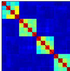
Hierarchical clustering
