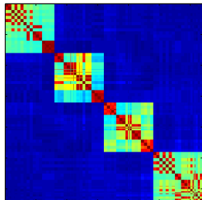
Classical scaling
