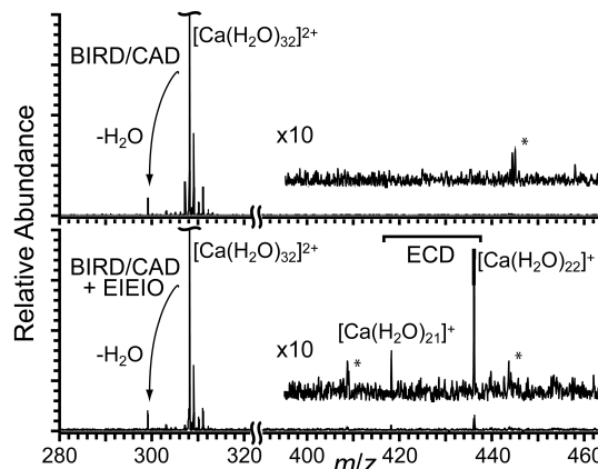
Figure 1. ECD spectrum of Ca(H_2O)_{32}^{2+} (bottom) showing reduced precursor ions that have lost 10 or 11 water molecules and reference spectrum (top) measured under identical conditions but with no electrons injected into the cell showing extent of BIRD and/or CAD that occurs.
