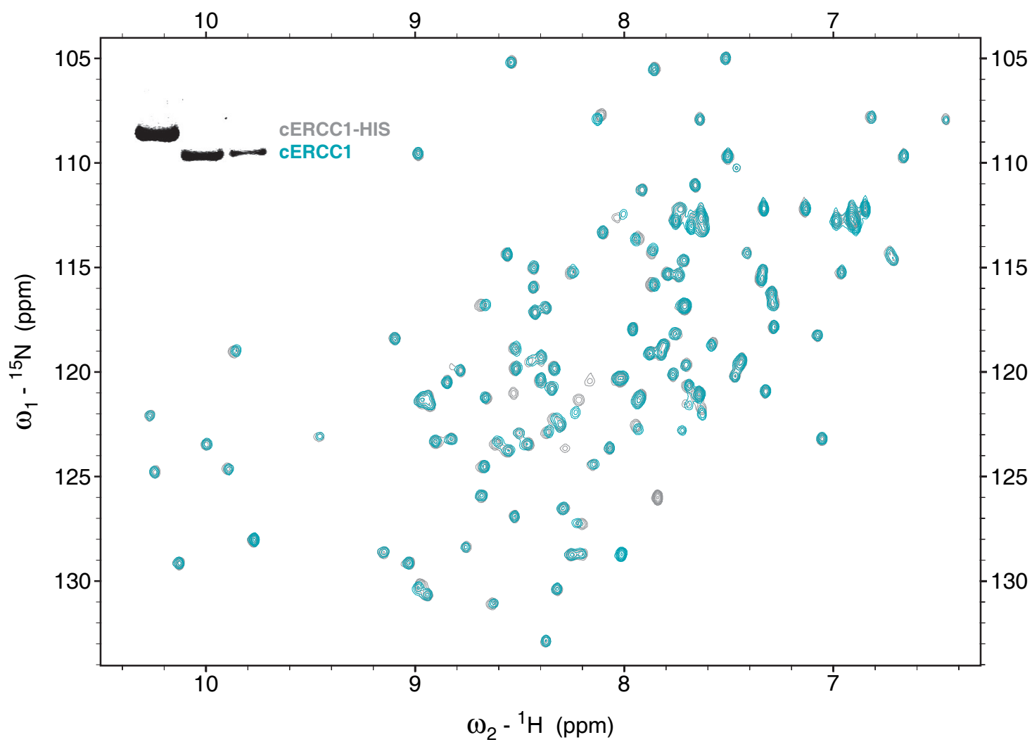
Supplementary Figure 1. ^1\text{H} - ^{15}\text{N} HSQC spectra of the C-terminal his-tag cERCC1 (gray) and the corresponding untagged protein (cyan). Inset shows the difference in mass for the two proteins.
