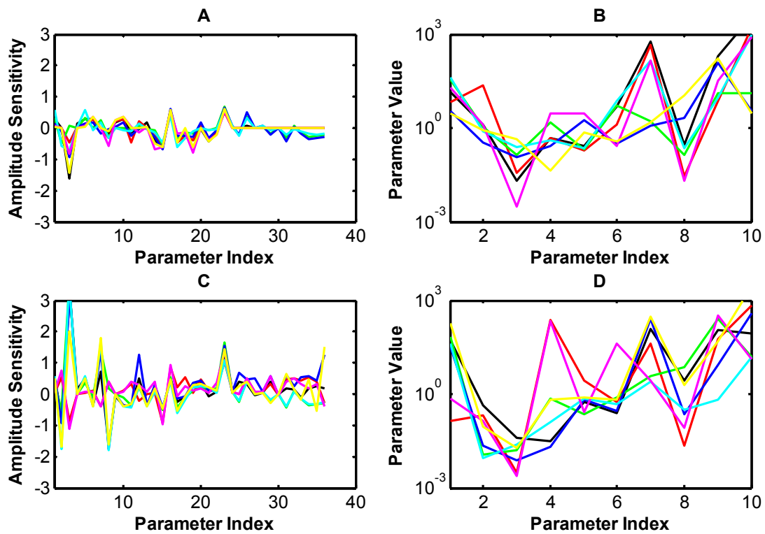
Figure S8 Distributions of amplitude sensitivities and their associated kinetic parameter values
