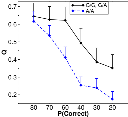
Q values fit to Test
