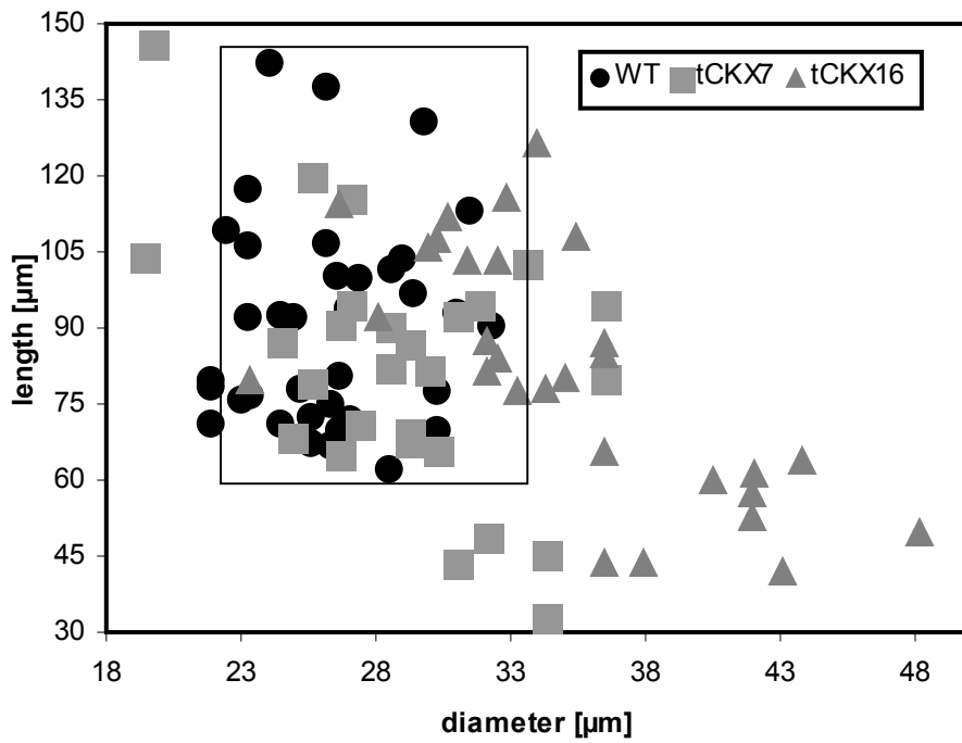
Figure S2. Cell dimensions of chloronema tissues of wild type (WT) Physcomitrella patens and the CKX transgenic lines tCKX7 and tCKX16, which form cells with increased diameters. The box indicates the ranges of dimensions obtained for WT cells.
