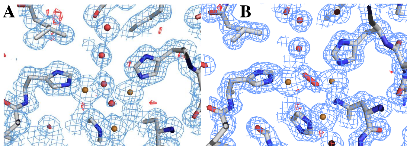
Figure 6 - (A) and (B) Representations of the 2Fo-Fc difference Fourier map (cyan colored, the electron density is contoured at 3\sigma ) with a superposed Fo-Fc difference Fourier map (red colored, The electron density is contoured at 3\sigma ), for the T2/T3 active site of molecules A and B of LtL respectively.
