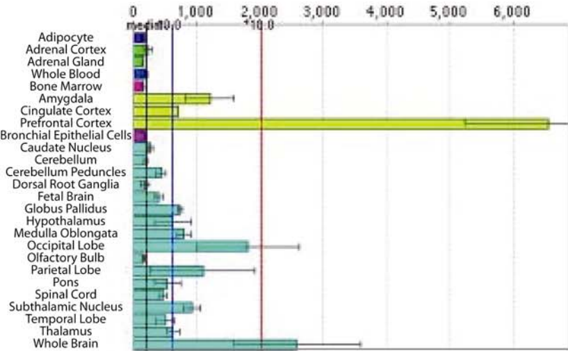
CNTNAP2 Reporter 219300_s_at Human GeneAtlas GNF1H, gcRMA
