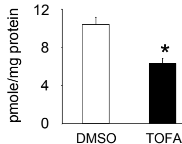
(C) ICV infusion of TOFA decreases hypothalamic malonyl-CoA level
