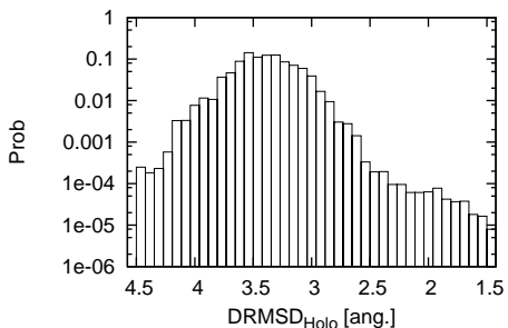
snapshot 100 \tau
