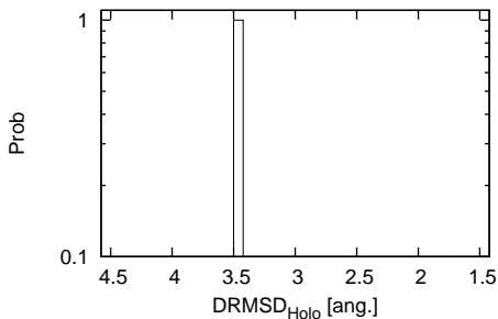
snapshot 4 \tau
