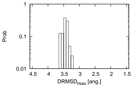
snapshot 8 \tau
