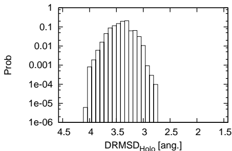
snapshot 16 \tau
