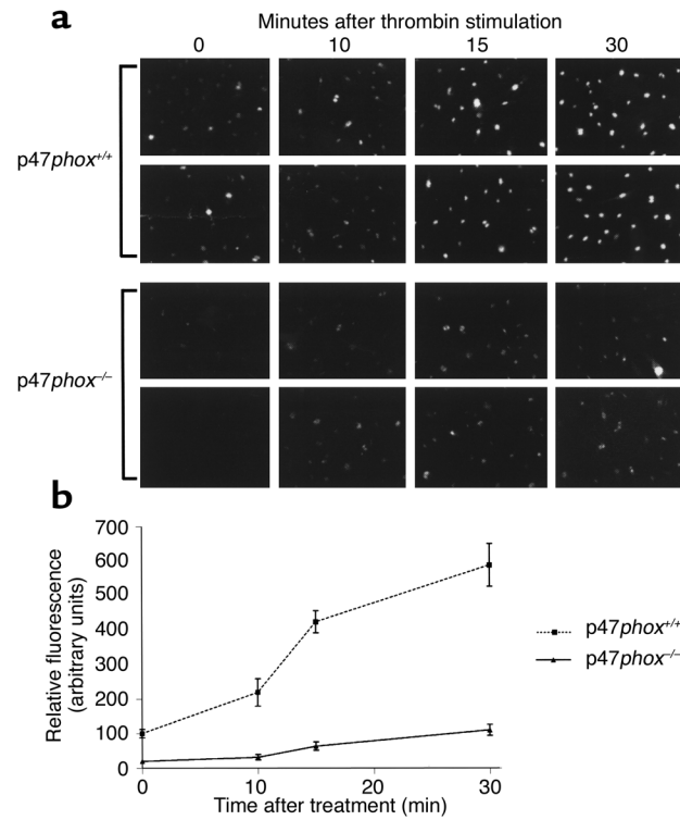
Figure 1 Detection of O_2^- by DHE in cultured SMCs. (a) SMCs from p47phox +/+ mice and p47phox -/- mice were treated with thrombin for the indicated time periods and incubated with DHE to detect O_2^- , as described in Methods. Representative panels are shown. (b) Fluorescence was quantified as described in Methods from cells treated in quadruplicate, and results are expressed as arbitrary units \pm SEM.
