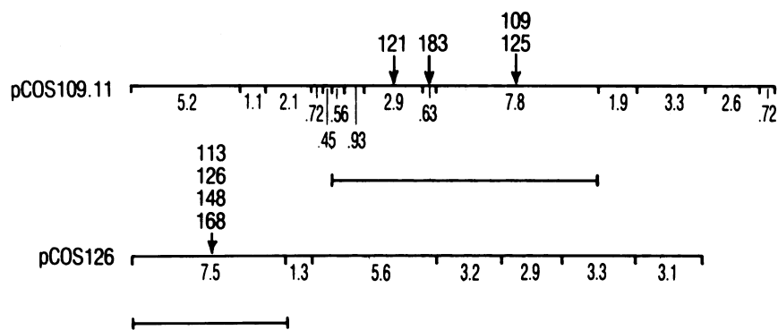
FIG. 5. Eco RI restriction maps of the rhizobial DNA of cosmids pCOS109.11 and pCOS126. Arrows indicate within which Eco RI restriction fragments the lps mutations are located as determined by complementation or hybridization. Horizontal lines below the restriction maps delineate subcloned DNA (pDEL23 and pE168) that complemented all four of the mutations in the respective regions. Numbers below the maps indicate sizes of Eco RI fragments in kilobase pairs.
