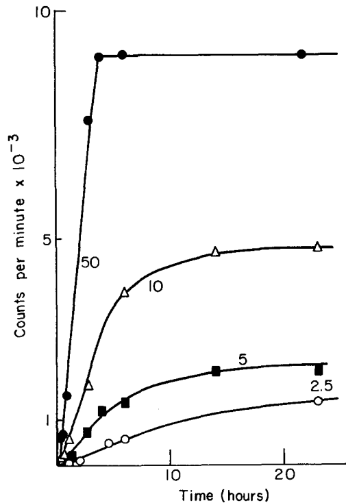
FIGURE 10 Incorporation of H^3 -colchicine versus time for colchicine concentrations of 50, 10, 5, and 2.5 \times 10^{-8} M. All data are expressed per 3 \times 10^6 cells.
