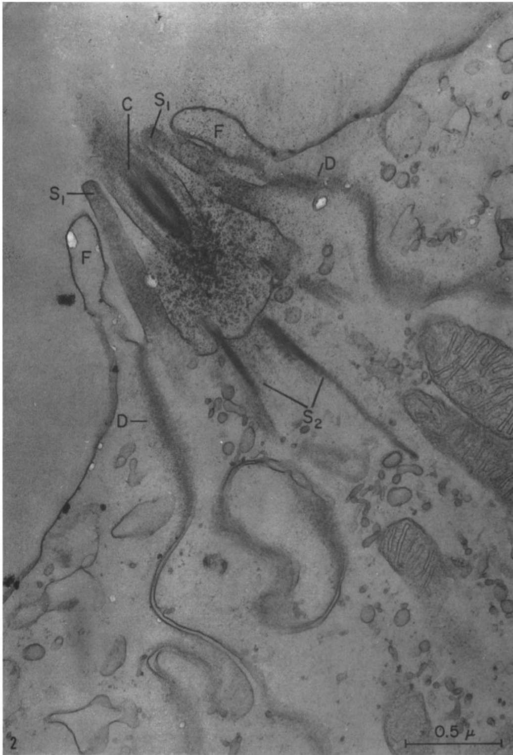
FIGURE 2 An oblique section through the endocil ( C ) region of a nematocyst. Outer long supports ( S 1 ) and inner, short, dense supports ( S 2 ) are seen along with a cell membrane fold ( F ) derived from adjacent cells. A periodicity of 100 Å is visible in the desmosomes ( D ). × 58,500.
