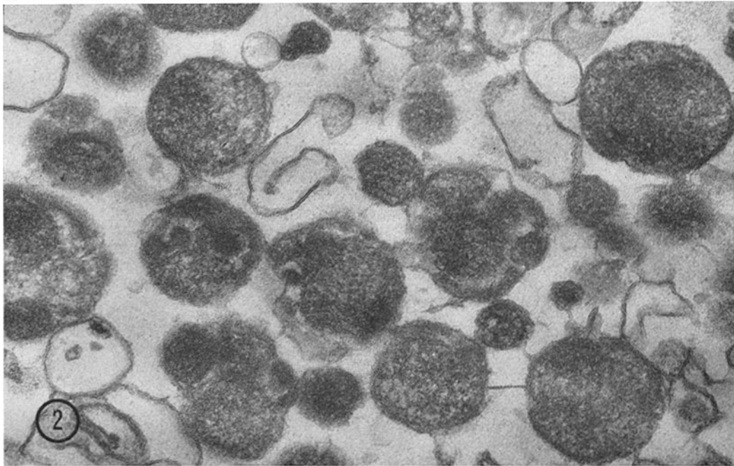
FIGURE 1 Portion of mitochondrial pellet obtained from wild type (YFp + ) cells. \times 46,000 .
