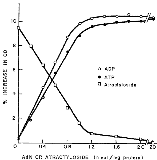
FIGURE 6 Estimation of the concentration of sites involved in inner membrane contraction induced by exogenous adenine nucleotide ( AdN ). Mitochondria of the study in which adenine nucleotide concentration was varied were suspended in media containing initially 250 mM sucrose, 10 mM K-PIPES (pH 6.4), 2.5 mM malate-pyruvate, and 1 mM EDTA. Bongkreikic acid (4 nmol/mg protein) was added after 1 min and adenine nucleotide after 2 min of preincubation. The OD changes given represent the maximum change in mitochondrial OD which occurred within 2 min after adding the bongkreikic acid. Mitochondria of the study in which atractyloside concentration was varied were suspended initially as described above except that atractyloside was present as indicated. The mitochondria were preincubated for 2 min and contraction was induced by adding 50 \mu M AOPCP.
