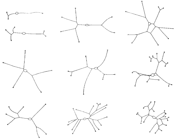
FIGURE 2 Outlines of a number of sympathetic neurons growing singly in culture. Bar, 100 \mu m.
