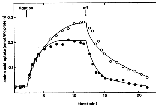
FIG. 6. Uptake of leucine (●) and lysine (○) in C. acetobutylicum membrane vesicles fused with RC-liposomes. Uptake was started by switching on the light ( 9.0 \text{ kW/m}^2 ) and terminated by switching the light off. [ ^{14}\text{C} ]leucine and [ ^{14}\text{C} ]lysine were added to final concentrations of 4.5 \mu\text{M} . Experiments were performed as described in Materials and Methods.
