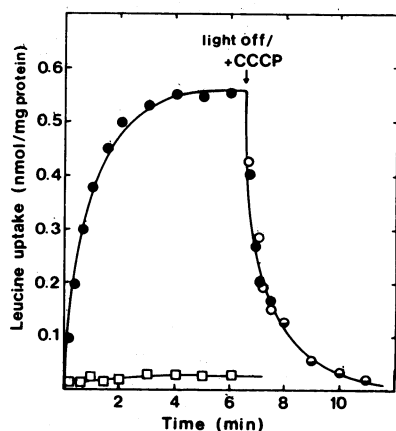
FIG. 2. Uptake of leucine by S. cremoris membrane vesicles fused with RC-liposomes. Experiments were performed as described in Materials and Methods at maximum light intensity ( 9.0 kW/m ^2 ). Uptake was started by adding [ ^{14}\text{C} ]leucine ( 4.5 \mu\text{M} ). At the arrow, the light was switched off (●) or CCCP ( 2 \mu\text{M} ) was added (○).
