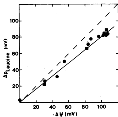
FIG. 4. Relationship between the accumulation level of leucine ( \Delta p_{\text{Leu}} ) and \Delta\psi in S. cremoris membrane vesicles fused with RC-liposomes. Data were collected as described in the legends to Fig. 2 (●) and Fig. 3 (■).
