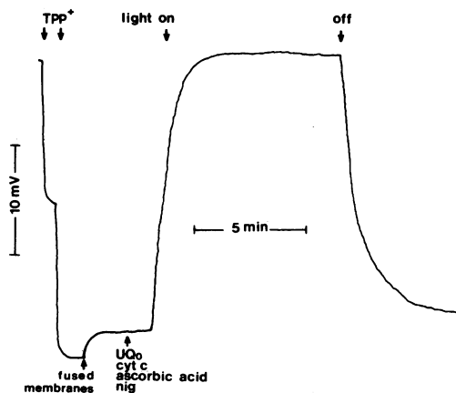
FIG. 1. Effect of illumination on the accumulation of TPP + in S. cremoris membrane vesicles fused with RC-liposomes. Experiments were performed in the presence of ubiquinone-0 (UQ 0 , 400 \mu M), cytochrome c (cyt c , 20 \mu M), ascorbic acid (500 \mu M), and nigericin (nig, 20 nM), as described in Materials and Methods.
