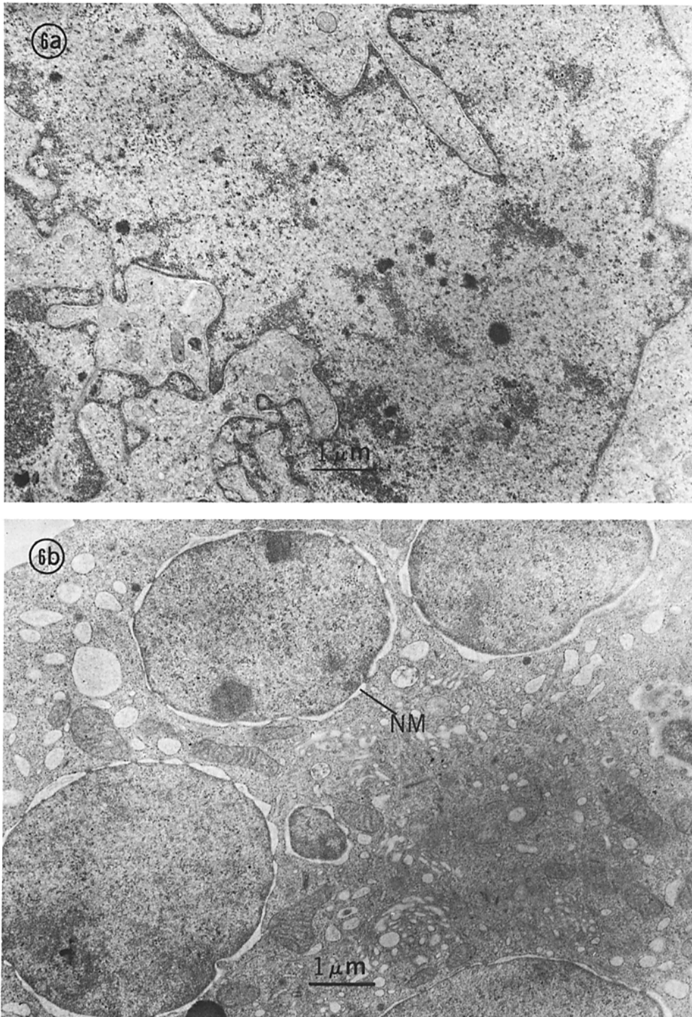
FIGURE 6 Electron micrographs of G_1 phase ZnCl_2 -pretreated cells. (a) Normal looking cells, \times 13,000 . (b) Cells with a swollen nuclear membrane (NM), \times 13,000 . G_1 phase ZnCl_2 -pretreated cells were prepared as described in Fig. 2.
