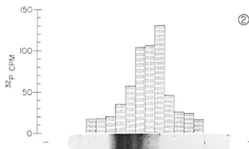
FIGURE 2 Incorporation of ^{32}P into slower moving bands of F_1 histone from ZnCl_2 -treated metaphase cells. ZnCl_2 -treated metaphase cells were prepared as described in the legend of Fig. 1, except that [ ^{32}P ]phosphate was added at the same time as ZnCl_2 .
