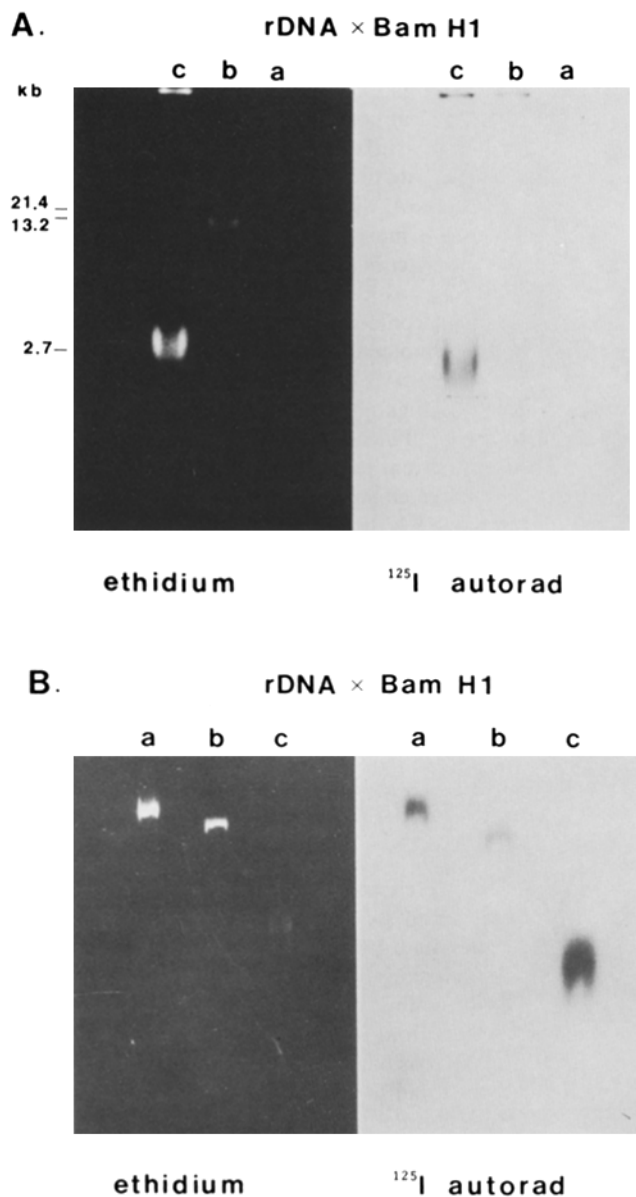
FIGURE 2 ^{125}\text{I} -labeled protein bound to Physarum rDNA restriction fragments. Labeling and purification of rDNA on two CsCl gradients was as described in Materials and Methods. The rDNA (5–10 \mu\text{g} ) was digested with Bam HI as previously described (4) and subjected to electrophoresis on 1.4% agarose gels containing 0.1% SDS. For panel A, bands were excised, and DNA extracted by electroelution was again subjected to electrophoresis on a 1.5-mm-thick agarose gel. On this gel, band c is overrepresented to enhance visibility. For panel B, excised bands were placed directly onto a second 1.4% agarose gel, and rDNA fragments are thus represented in equimolar quantities. Gels were dried and autoradiographed using Dupont Cronex film and an intensifying screen for 7 d at -80^\circ . Note that the bulk of protein label is in the Bam c terminal restriction fragment even though this fragment contains <10\% of the total rDNA.
