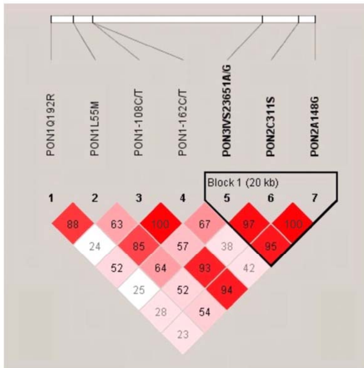
Supplementary Figure. Haploview plots of pairwise LD across the PON gene cluster. Panel A shows values for r^2 \times 100 . The two-locus haploblock comprising SNPs 2 and 5 shows low correlation ( r^2=0.32 ). Panel B shows values for D' \times 100 . A block of high LD across PON2 and PON3 is illustrated.
