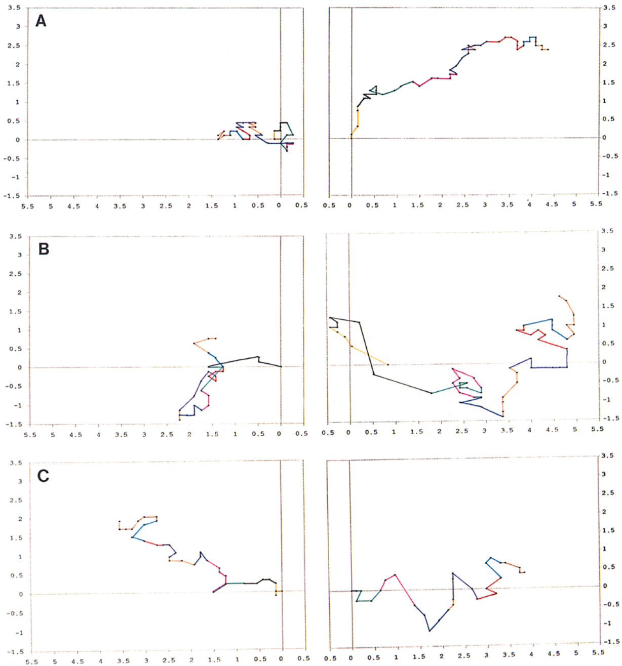
Figure 4. Two-dimensional space-time plots of the separating centrosomes in the prophase (A), ALP (B) and anaphase (C) cells shown in Figs. 3, 5, and 6, respectively. Each plot consists of left- (centrosome No. 1) and right- (centrosome No. 2) hand sides which together depict the displacement of both centrosomes during the same 4-min 40-s interval. The plot for each centrosome starts at the 0 intersect of the X and Y axes, and each is subdivided into ten consecutive color-coded segments. Each of these segments documents the X and Y motion, in micrometers, of that centrosome over seven 4-s frames. Matching colors in the left- and right-hand sides reflect the same time period. Colored segments containing less than seven data points, or missing segments, reflect that the centrosome was stationary for one or more time points. See text for details.
