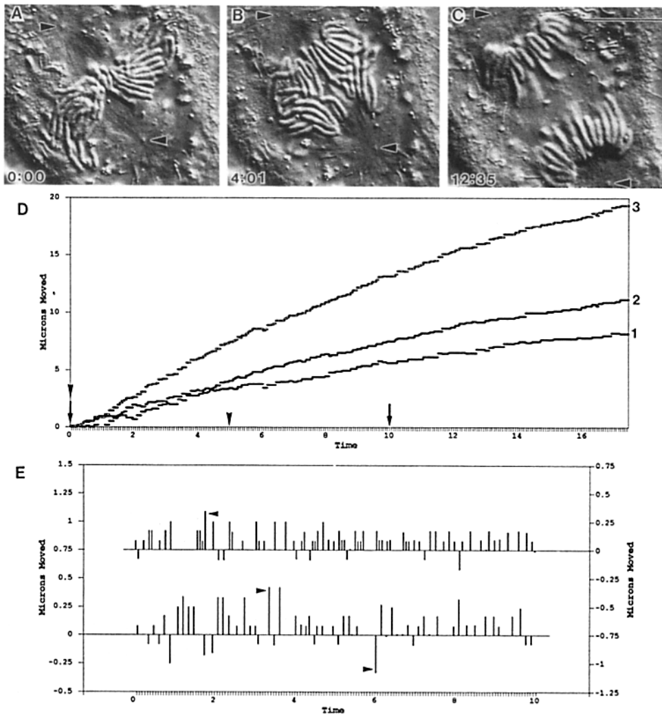
Figure 6. (A-D) Exactly as in Fig. 3 except these centrosomes are in an anaphase cell. Arrowheads along the time axis in (D) note that time period covered by the two-dimensional space-time plot in Fig. 4 C. Bar (C), 20 \mu\text{m} .
