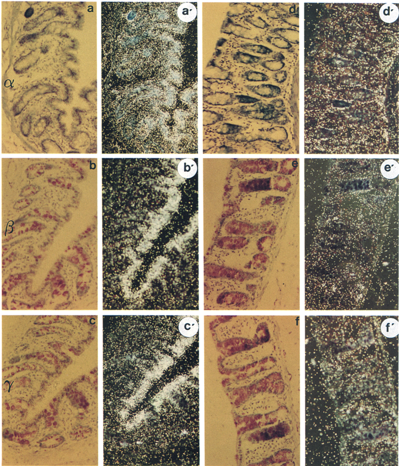
Figure 7. Expression of \alpha , \beta , and \gamma rENaC subunit mRNA in the distal colon. Sections were hybridized with antisense probes specific for the \alpha subunit mRNA (a and a'), the \beta subunit mRNA (b and b'), the \gamma subunit mRNA (c and c'), or with sense probes for \alpha (d and d'), \beta (e and e') or \gamma (f and f') subunits. Each section is shown as bright field and as dark field photograph (ex: a and a', respectively). All three subunit mRNAs are strongly expressed in the most superficial cells of the distal colon epithelium, while crypt cells are negative. A uniform and low labeling was observed with the sense probes, contrasting with the intense signal observed with the antisense probes. Magnification: \times 200 . Bar, 100 \mu\text{m} .
