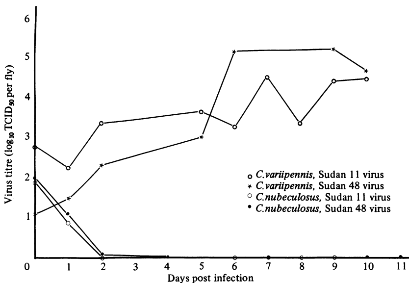
Fig. 4. Replication of Sudan 11 and Sudan 48 viruses in C. variipennis and incubation of the viruses in C. nubeculosus after oral ingestion.
