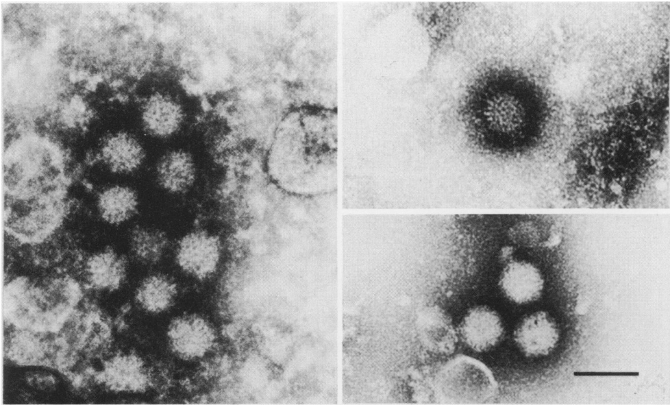
Fig. 2. Electron micrograph of Sudan 48 virus particles. Barline 100 nm. Particle size 70 nm.
