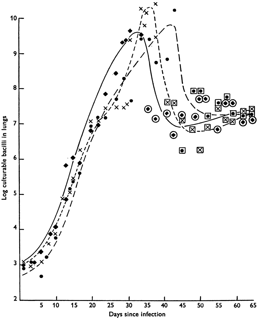
Fig. 2. Comparison of culturable lung counts in relation to duration of infection and foot-pad sensitivity to tuberculin in three strains of mice. ●—● C57 strain—highly susceptible; ×—×, H.I. strain—moderately susceptible; ◆—◆, M.U.A. strain—resistant; □ ☒ ⊙, animals showing positive tuberculin reaction.
