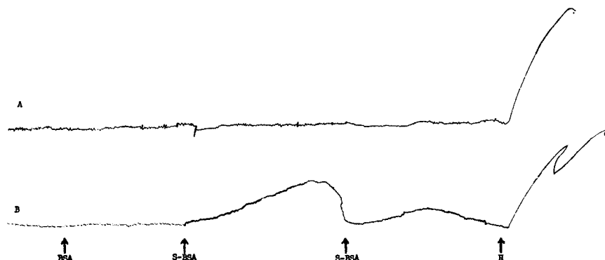
FIG. 7. A kymograph record of the Schultz-Dale responses in guinea pigs obtained with the salt fractions of the antigen material. Sensitization was with the equivalent of 0.1 mg. of antigen based on radioactivity. Test antigen added was 10 mg./150 ml. bath and histamine added was 5 \mu g. (A), salt-insoluble fraction, indicating no sensitization; (B), salt-soluble fraction, demonstrating sensitization.
