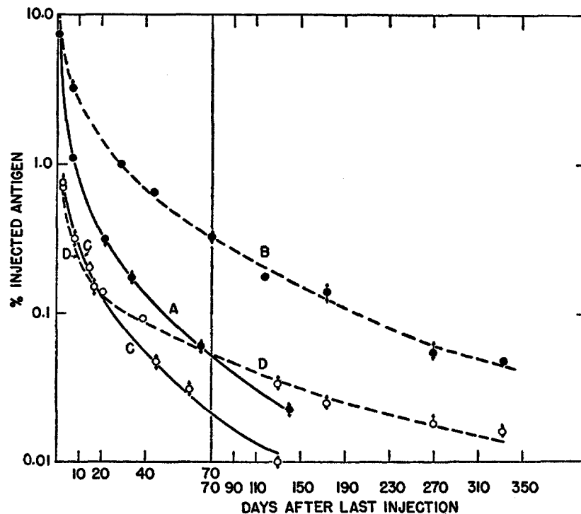
FIG. 4. Semilog plot of the retention in perfused liver tissue of a single injection of 50 mg. S^{35} -BSA (A); a single injection of 50 mg. S^{35} -KLH (B); multiple injections i.e. 9 of 10 mg. each of S^{35} -BSA (C); and multiple injections i.e. 9 of 10 each of S^{35} -KLH (D). The center of the circles indicates the mean of the distribution which is indicated by the arrows.
