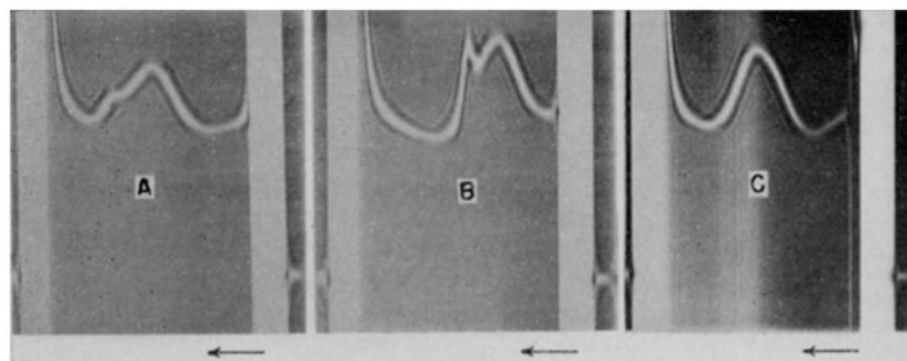
FIG. 8. Sedimentation boundaries of the salt-soluble fraction obtained from tissue removed 21 days after a single injection of 10 mg. S 35 -BSA (A); salt-soluble fraction obtained from tissue removed 21 days after 9 injections totaling 90 mg. of S 35 -BSA (B); and salt-insoluble fraction obtained from tissue removed 21 days after single injection of 10 mg. S 35 -BSA (C).
