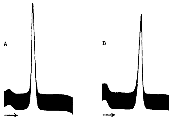
FIG. 1. Electrophoresis diagrams of (A) BSA and (B) S-BSA at 1 per cent protein concentration in barbital buffer at pH 8.6, \mu = 0.1 . Migration was for 1 hour in the descending limb with the direction of migration indicated by an arrow.
