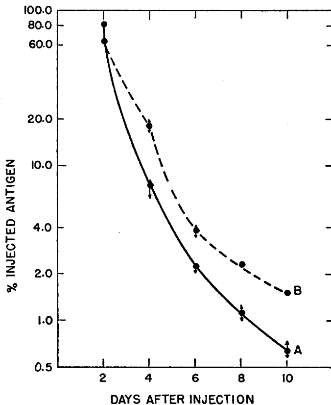
FIG. 6. A semilog plot of urine-excreted radioactivity when either 10 mg. of S 35 -BSA or S 35 -KLH was given intravenously. The center of the circles indicates the mean of the distribution which is indicated by the arrows.
