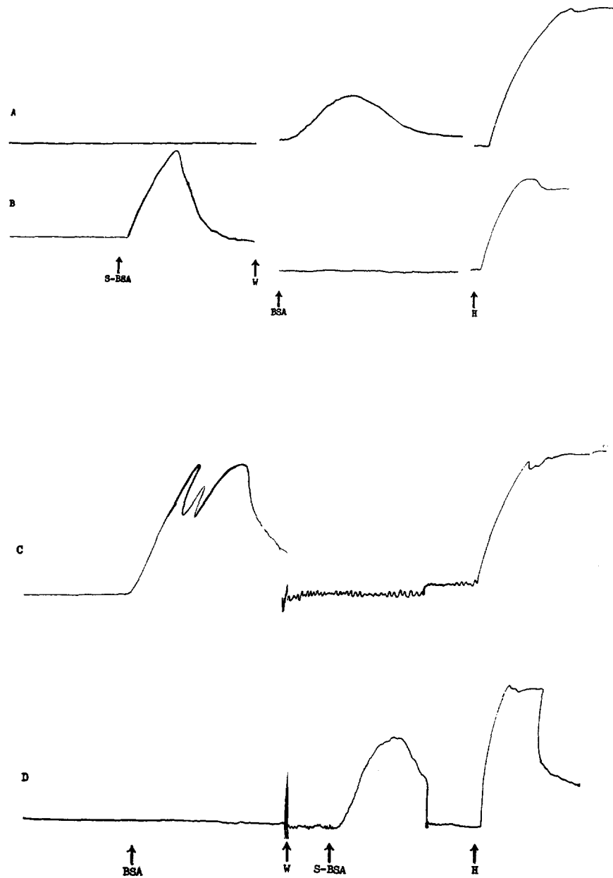
FIG. 3. Kymograph records of the specific reaction of BSA and S-BSA antigens following active sensitization of guinea pigs with 20 to 30 mg. protein. Muscle strips were 3 to 6 cm. from the cecum and the concentration of test antigen was 5 mg./150 ml. tissue bath. W , washing; H , 5 \mu g. histamine. (A), sensitized with 20 mg. BSA; (B), sensitized with 20 mg. S-BSA; (C), sensitized with 20 mg. BSA; (D), sensitized with 20 mg. S-BSA.
