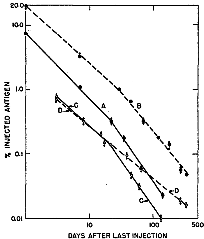
FIG. 5. Retention of single and multiple injections of S^{35} -BSA and S^{35} -KLH, using the same data as in Fig. 4 but as a log-log plot. The center of the circles indicates the mean of the distribution which is indicated by the arrows.
