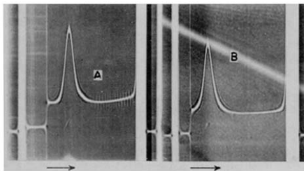
FIG. 2. Sedimentation patterns after 18 minutes for (A) BSA and 16 minutes for (B) S-BSA at 59,780 R.P.M. 1 per cent protein solutions were used with the diluent of 1 per cent NaCl being used to form a boundary in a synthetic boundary cell.
