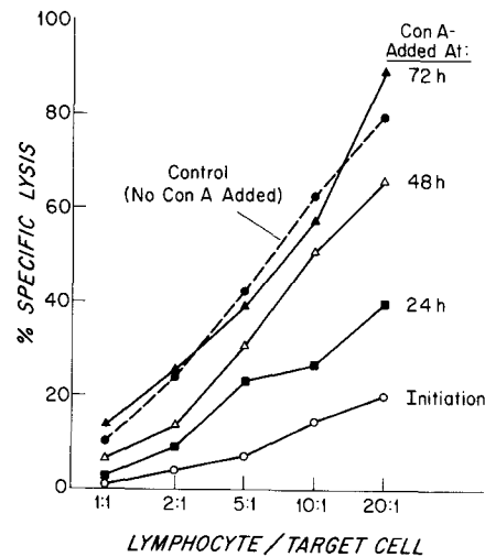
FIG. 2. Effects of adding soluble Con A at intervals after culture initiation on cytotoxic responses in vitro. 2 \mu g Con A/ml were added to the MLC of C57BL/6 and mitomycin C-treated DBA/2 spleen cells at initiation or 24, 48, and 72 h thereafter. ^{51}\text{Cr} -release assays were performed on day 5 using P815 mastocytoma as target cells.
