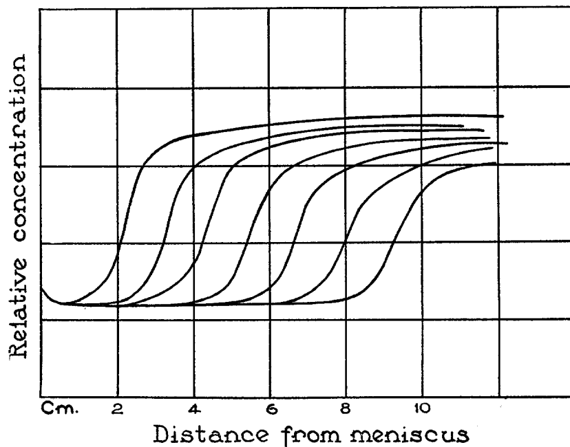
FIG. 3. Photometer curve of run 17.
