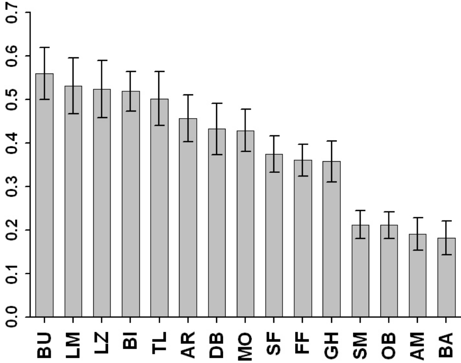
Mean ( \pm SE) correlation coefficient with other taxa
