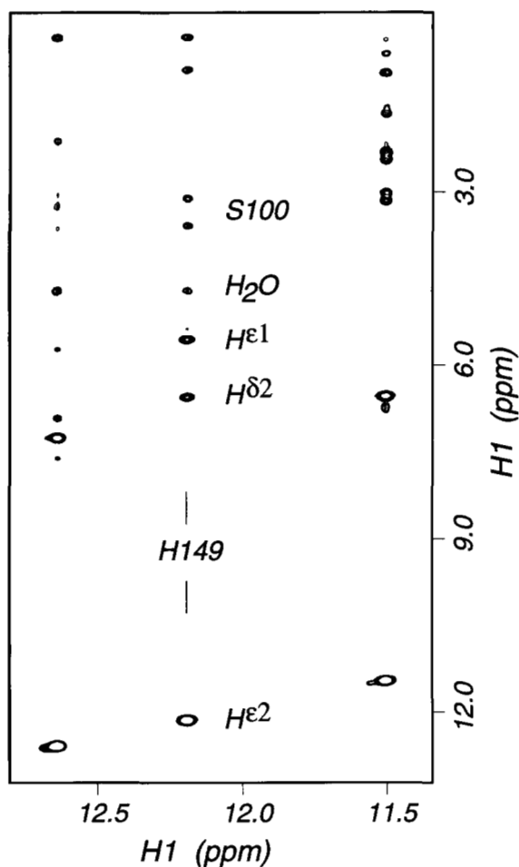
Fig. 5. Portion of the NOESY spectrum of BCX ( \tau_{\text{mix}} = 150 ms) recorded with a gradient 11-echo detection pulse sequence tuned for the ^1\text{H}^{\epsilon 2} of His 149 (Sklenár & Bax, 1987). Assignment of the tautomeric state of His 149 is confirmed by NOE cross peaks between ^1\text{H}^{\epsilon 2} and the adjacent carbon bonded ^1\text{H}^{\delta 2} and ^1\text{H}^{\epsilon 1} of this residue, as well as by the absence of NOEs to its ^1\text{H}^{\beta, \beta'} (Plesniak et al., 1996). NOE cross peaks to the ^1\text{H}^{\beta} and ^1\text{H}^{\beta'} of nearby Ser 100 are also labeled. A cross peak at the frequency of \text{H}_2\text{O} is tentatively assigned to a NOE interaction with a buried water that is hydrogen bonded to \text{N}^{\epsilon 2}\text{H} of His 149 or to the \text{O}^{\gamma}\text{H} of Ser 100. The diagonal peaks at 11.5 and 12.6 likely arise from the phenolic \text{O}^{\gamma}\text{H} of tyrosines.
