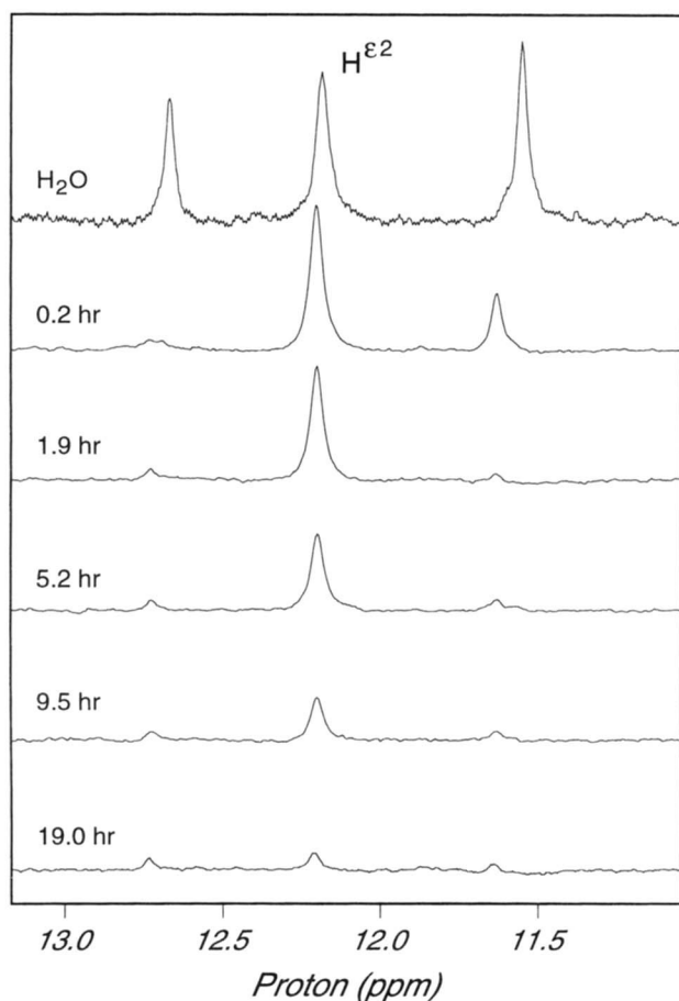
Fig. 6. Time course of the hydrogen–deuterium exchange of the ^1\text{H}^{\epsilon 2} of His 149 at 30 °C and \text{pH}^* 7.04 . The top spectrum corresponds to BCX in \text{H}_2\text{O} buffer, whereas the descending spectra were recorded after transfer into \text{D}_2\text{O} , with data acquisition started at the indicated times. Small peaks in the final spectrum result from \sim 5\% residual HDO in the solvent.
