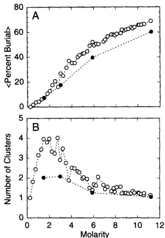
Fig. 6. Box volume comparison. Simulations using our standard reference box volume shown by open circles (connected by a dotted line) are compared to the four simulations at half the box volume but the same concentration shown by filled circles (connected by a broken line). Concentrations of all simulations shown in terms of their molarity. Note that the simulations at half the box volume contain half the number of solutes (methane) and water molecules (see Table 2). A: Mean burial. B: Number of clusters.
