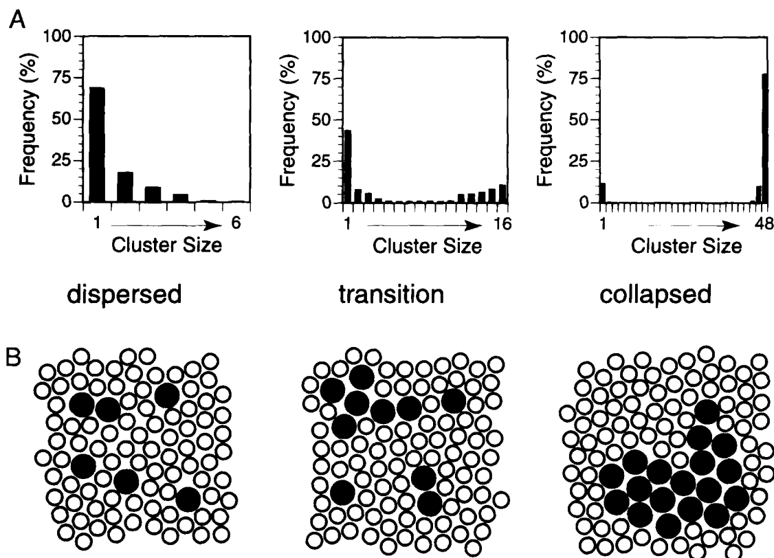
Fig. 7. Three stages of solute aggregation. A: Cluster distributions from representative methane simulations in each of the three stages. For the dispersed stage, we show the distribution from the 6-methane simulation, which clearly favors the solvated species. The distribution illustrative of the transition stage was calculated from the 16-methane simulation, which clearly shows the two overlapping populations located at the two extremes of the distribution. The existence of individual smaller clusters of solute molecules shows that the single aggregate is unstable. The distribution illustrative of the collapsed stage was calculated from the 48 methane simulation, which shows two populations well-separated from each other. None of the intermediate cluster sizes are populated. B: In two dimensions, we depict our interpretation of the three stages found in our simulations. These illustrations were made after extensive viewing of the simulations using space-filling representations of the moving solute molecules in stereographics. Free solute dominates the dispersed stage; some molecules do aggregate, but no large clusters form. We also find some existence of the solute separated pair as shown by the two solutes in the lower left-hand corner of the box. The transition stage cycles between the large, single cluster and a state with several clusters of intermediate sizes. The final collapsed stage has only one cluster, the stable hydrophobic aggregate. In the methane simulations, we would also find a single molecule solvated in solution, and for isobutylene molecules, there is only the single cluster.
