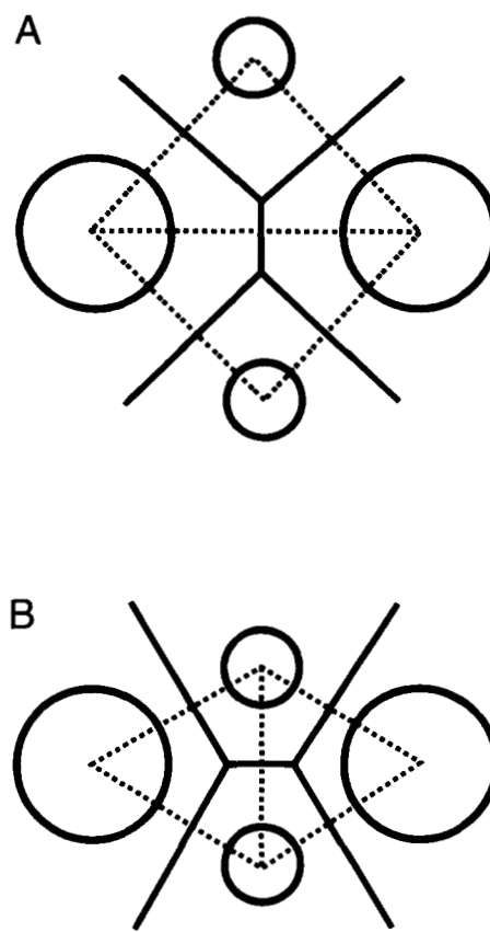
Fig. 2. Neighbors. A: Four atoms are shown by the spheres. Dark lines represent polyhedra faces shared between atoms and broken lines show the Delauney Tessellation. The two large atoms are in contact and occlude the small atoms from touching. B: Same as A, but the two small atoms are moved in closer so that they are now in contact (the Delauney Tessellation clearly shows this as do the polyhedra faces). Although the two larger atoms have not moved from the previous example, they are no longer in contact. Therefore, the two smaller atoms have affected the contact of the two larger atoms without changing the larger atoms' distance of closest approach.
