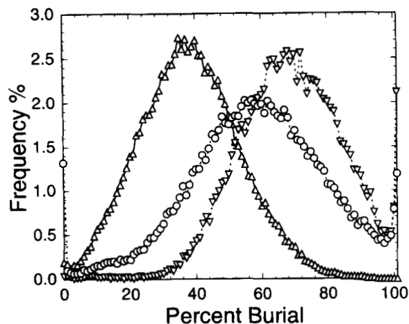
Fig. 3. Burial of solutes. Distributions of percent burial (as defined in the caption to Fig. 1) are shown for simulations containing 32 solute molecules of urea (triangles on a solid line, 6.71 M concentration), isobutylene (inverted triangles on a dashed line, 5.84 M concentration), and methane (circles on a dashed line, 7.83 M concentration).
