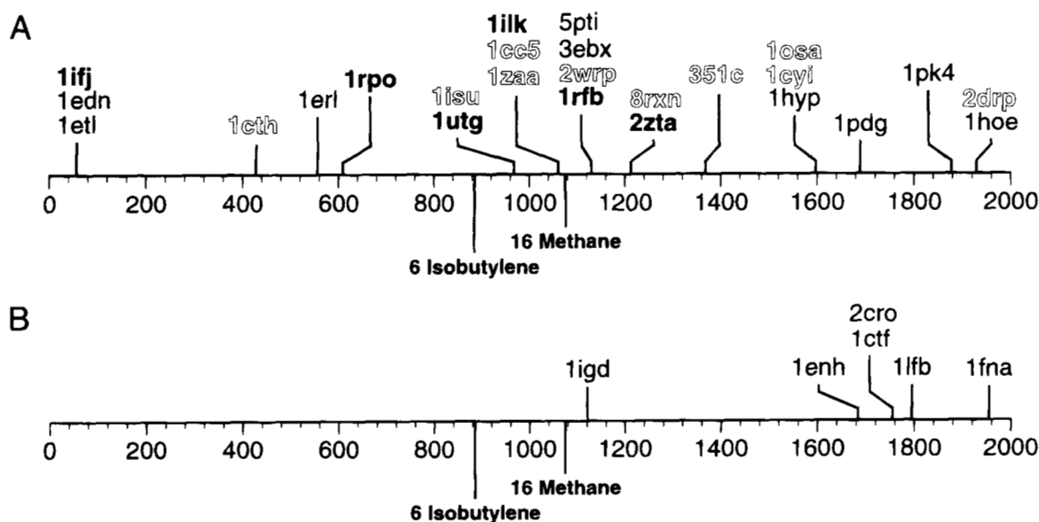
Fig. 8. Comparison with protein core volumes to minimal cluster volumes. To make the plot clearer, we placed all proteins possessing volumes within \sim 25 \text{ \AA}^3 of each other on the same point. The volumes for the minimum stable hydrophobic aggregate from the 16-methane ( 1,075 \text{ \AA}^3 ) and the 6-isobutylene ( 885 \text{ \AA}^3 ) simulations are also shown in both parts. A: Proteins using extra types of stabilization are shown. Depending upon which type of interaction they possess, we classify the proteins as follows: (1) with disulfides (in italics,) (2) oligomers (in bold), and (3) with prosthetic groups (in outline). B: We show proteins without any sort of additional stabilization.
