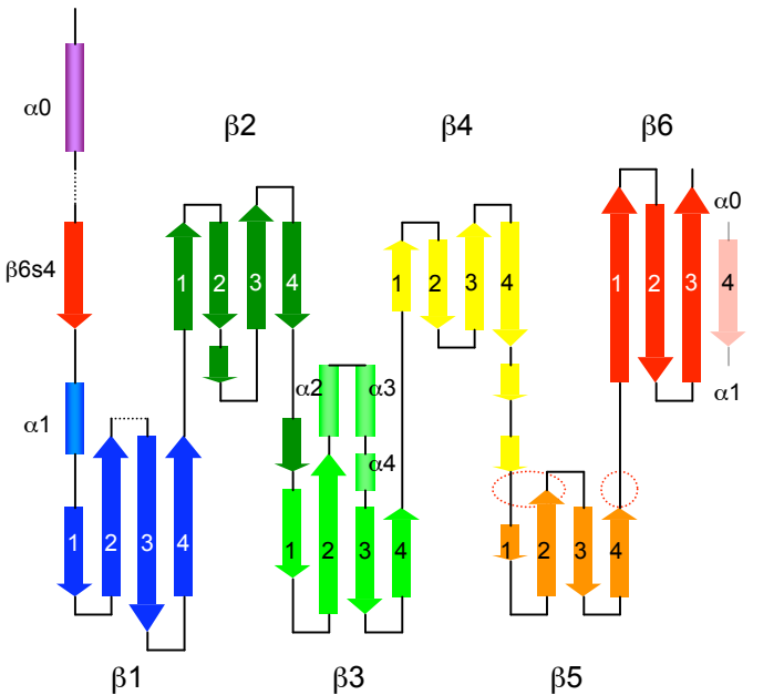
Putative SLAM-binding sites
