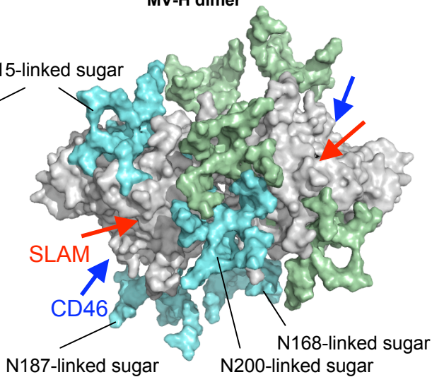
MV-H dimer
