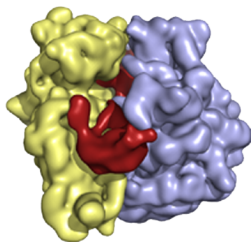
70S·IF2
