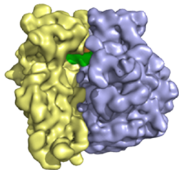
70S
