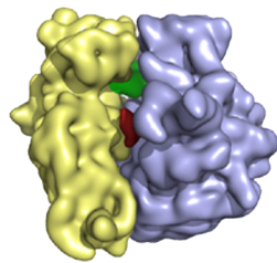
70S·RRF
