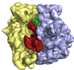
70S·EF-G
