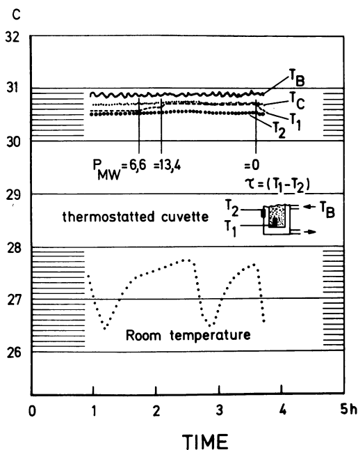
FIG. 2.—Plotter trace of differently registered temperatures. ( T_B thermostatted bath; T_C , control cuvette; T_1 , surface of the irradiated cuvette; T_2 , cuvette housing; \tau = (T_1 - T_2) is proportional to the absorbed microwave power.)
