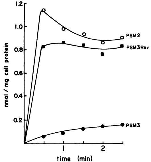
FIG. 1. Transport of 2 \mu\text{M} glutamine by PSM2, PSM3, and PSM3Rev, a revertant of PSM3.
