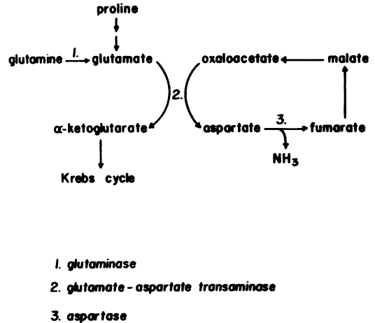
FIG. 7. The principal pathway of the catabolism of glutamate in E. coli , adapted from Marcus and Halpern (21).
