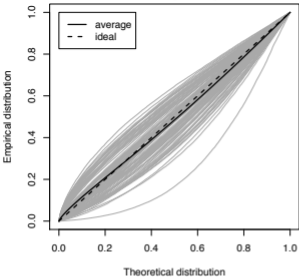
Ordinary Linear Model (Atrium)
