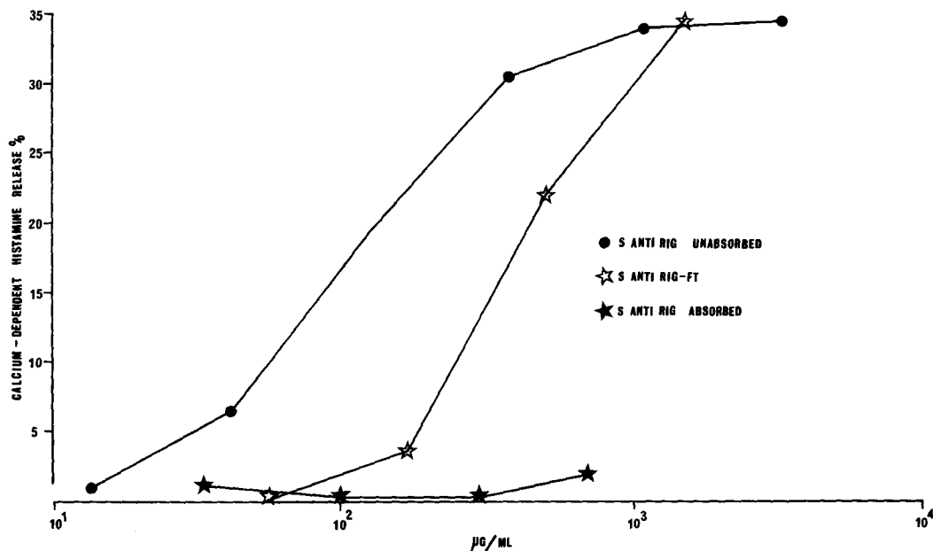
FIG 1. Dose-response curves for divalent S anti-RIg. \text{Ca}^{2+} -dependent ligand-induced histamine release is expressed as percent of the total cell histamine content. Calcium-independent release was in the range 1–6% and was not significantly different from spontaneous release. Absorption of S anti-RIg was with rat IgG linked to Sepharose.
