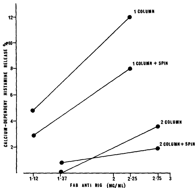
Fig. 2. Dose-response curves for monovalent Fab anti-RIg, showing progressive reduction in histamine release as a consequence of treatments designed to remove aggregates.
