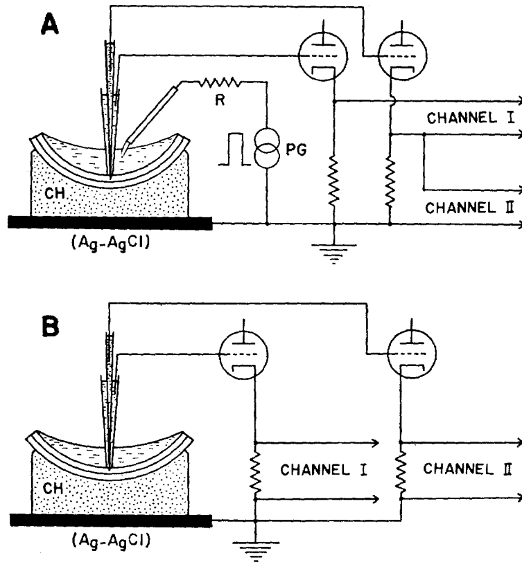
FIGURE 1. Arrangements for measurement of the radial resistance of the opened eye, A ; and for recording of responses to light, B . CH , Ringer-soaked chalk; PG , square pulse generator; R , 1 M \Omega resistance as a current limiter. See text.
