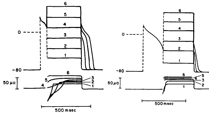
FIGURE 3. Membrane currents during clamps to different voltage levels. Left, clamp initiated 50 msec from onset of action potential; right, clamp initiated 225 msec from onset of action potential.
