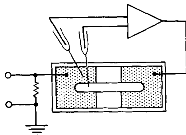
FIGURE 1. Block diagram showing myocardial preparation and voltage-clamp circuit.
