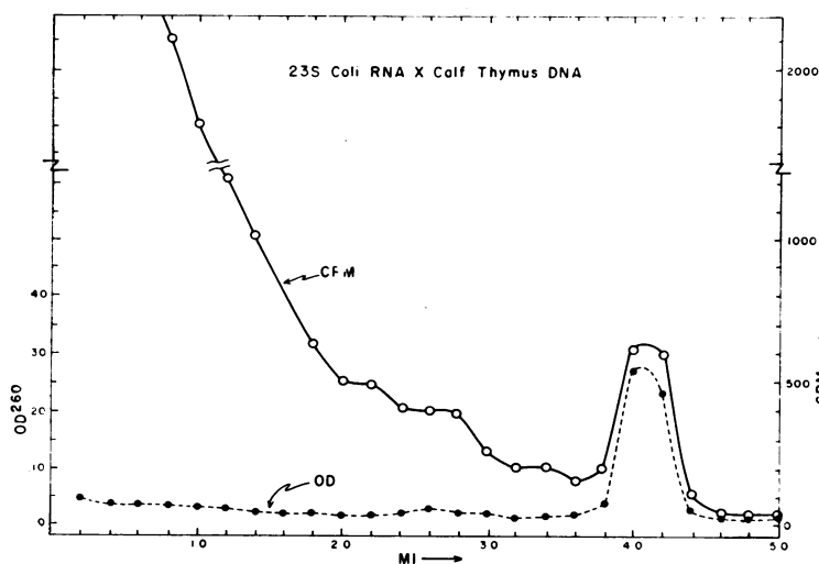
FIG. 3.—CsCl density gradient profile. 84 \mu\text{g}/\text{ml} heat-denatured calf-thymus DNA + 3.4 \mu\text{g}/\text{ml} 23S- \text{H}^3 -RNA ( 4.8 \times 10^4 cpm/ \mu\text{g} ) in TMS; slow-cooled from 55°C to 32°C. Centrifugation, at 33,000 rpm and 25°C, for 74 hr.
