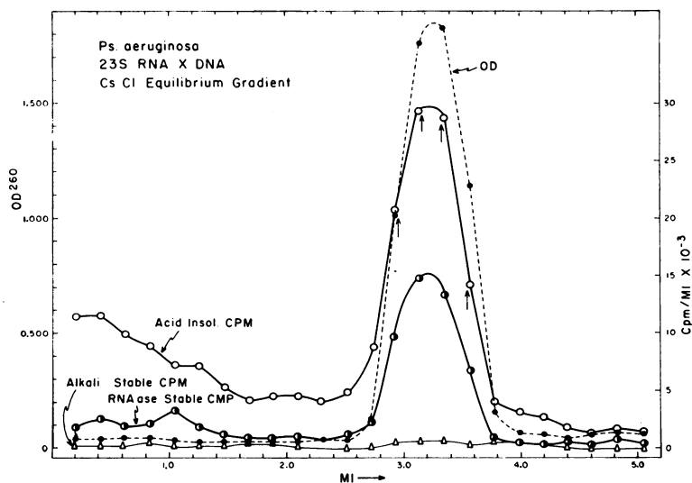
FIG. 1.—Cesium chloride equilibrium density gradient. 800 \mu\text{g/ml} Ps. aeruginosa heat-denatured DNA + 2.95 \mu\text{g/ml} 23S- \text{P}^{32} -RNA ( 6 \times 10^5 cpm/ \mu\text{g} ) in TMS slow-cooled from 55°C to 34°C. Duration of the centrifuge run was at 33,000 rpm and 25°C for 72 hr. 0.21 ml fractions collected and diluted 1.1 ml in TM buffer. Aliquots were directly taken for digestion with 5 \mu\text{g/ml} RNAase at 37°C for 30 min or 0.3 M NaOH at 30°C for 20 hr.
