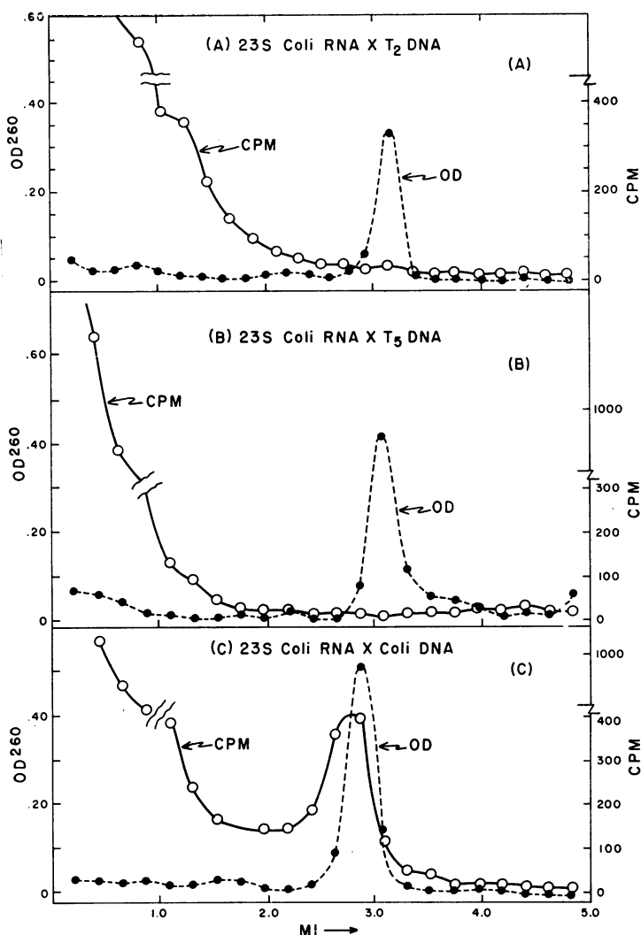
FIG. 2.—CsCl density gradient profiles. (A) 76 \mu\text{g/ml} T2 heat-denatured DNA + 3.4 \mu\text{g/ml} E. coli 23S- \text{H}^3 -RNA ( 4.8 \times 10^4 cpm/ \mu\text{g} ) in TMS. (B) 76 \mu\text{g/ml} T5 heat-denatured DNA + 3.4 \mu\text{g/ml} E. coli 23S- \text{H}^3 -RNA ( 4.8 \times 10^4 cpm/ \mu\text{g} ) in TMS. (C) 84 \mu\text{g/ml} E. coli heat-denatured DNA + 3.4 \mu\text{g/ml} 23S- \text{H}^3 -RNA ( 4.8 \times 10^4 cpm/ \mu\text{g} ) in TMS. All three reaction mixtures were held at 40°C for 36 hr. Centrifuge was at 33,000 rpm and 25°C for 72 hr.
