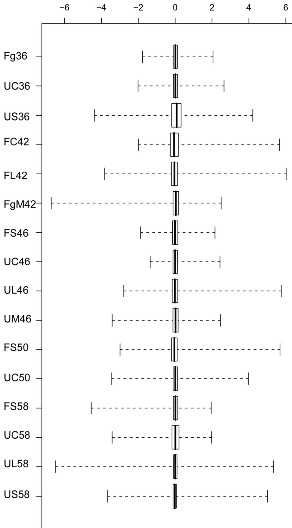
Boxplots of Relative M values
