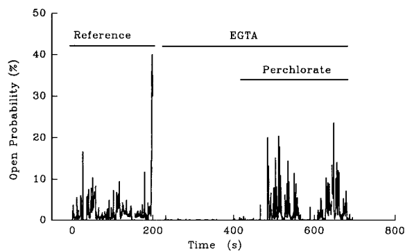
FIGURE 7. Effect of \text{ClO}_4^- on RyR open probability. Diary plot of the experiment of Fig. 6. Plotted are values of \bar{P}_o , evaluated as fractional open time during successive 2-s sweeps. The horizontal bars represent in time the presence of \text{ClO}_4^- and EGTA.
