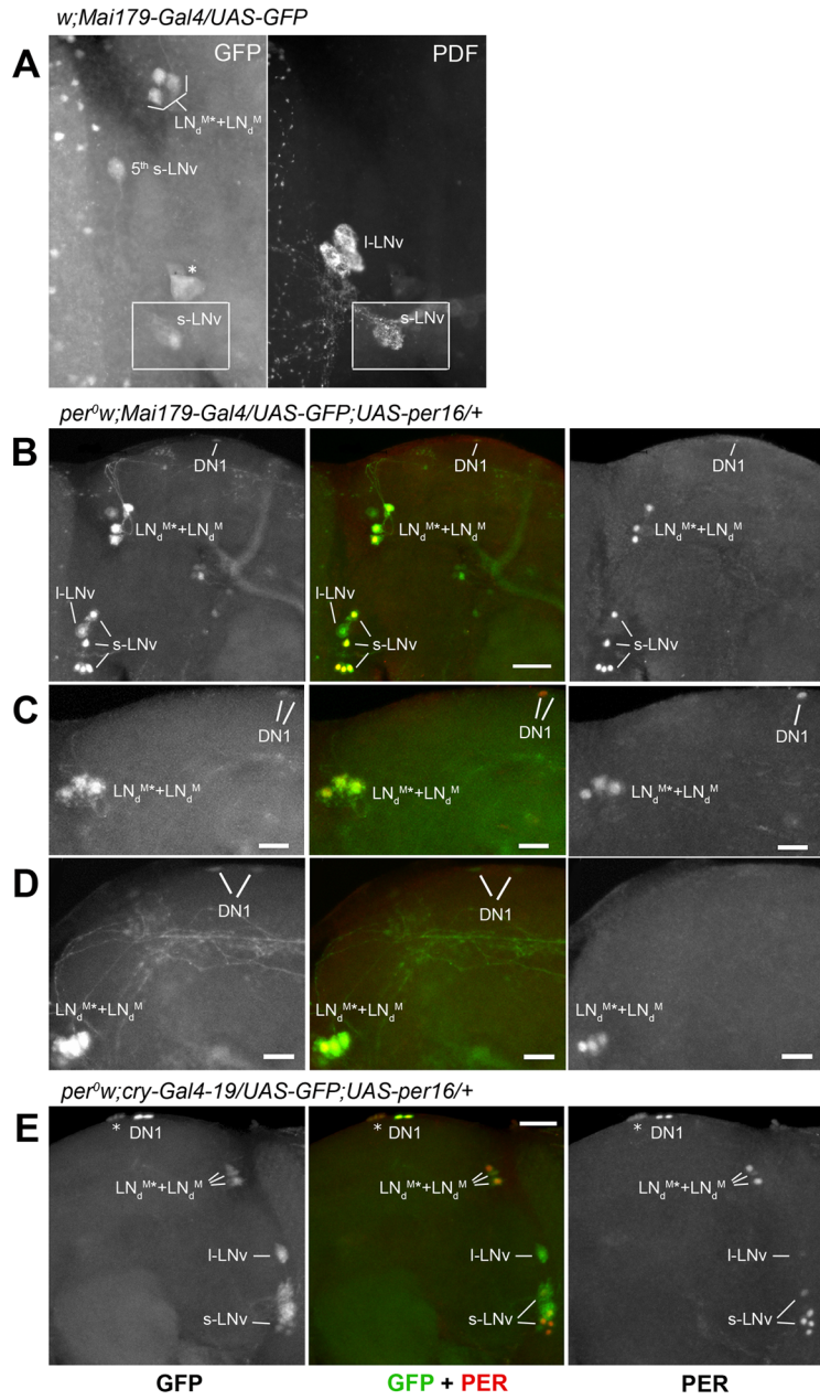
Supplementary Fig. 1 : Characterization of the Mai179-Gal4 and cry-Gal4-19 expression patterns
