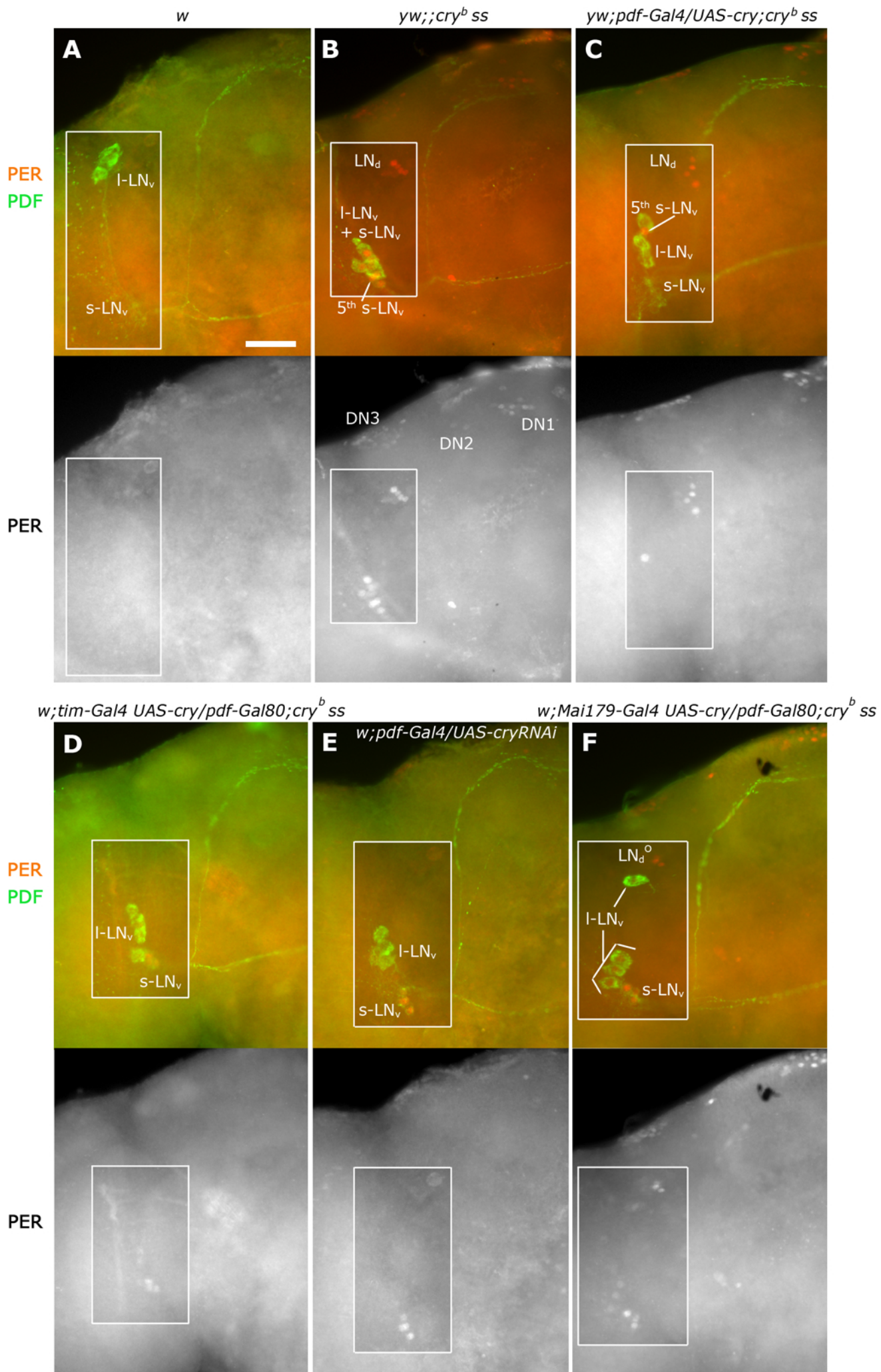
Supplementary Fig. 2 : Oscillator-autonomous inhibition of PER accumulation by CRY in LL
