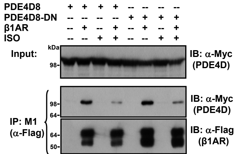
Supplementary Figure 5 Formation and agonist-dependent dissociation of \beta_1 AR/PDE4D complexes occurs whether the PDE4D is catalytically active or inactive. Exogenous \beta_1 AR was co-immunoprecipitated with a catalytically active PDE4D construct (PDE4D8) or a catalytically inactive PDE4D construct (PDE4D8-DN) from extracts of Hek293 cells that had been pre-treated for 15 min with or without 10 \mu M Isoproterenol (ISO). A representative experiment is reported.
